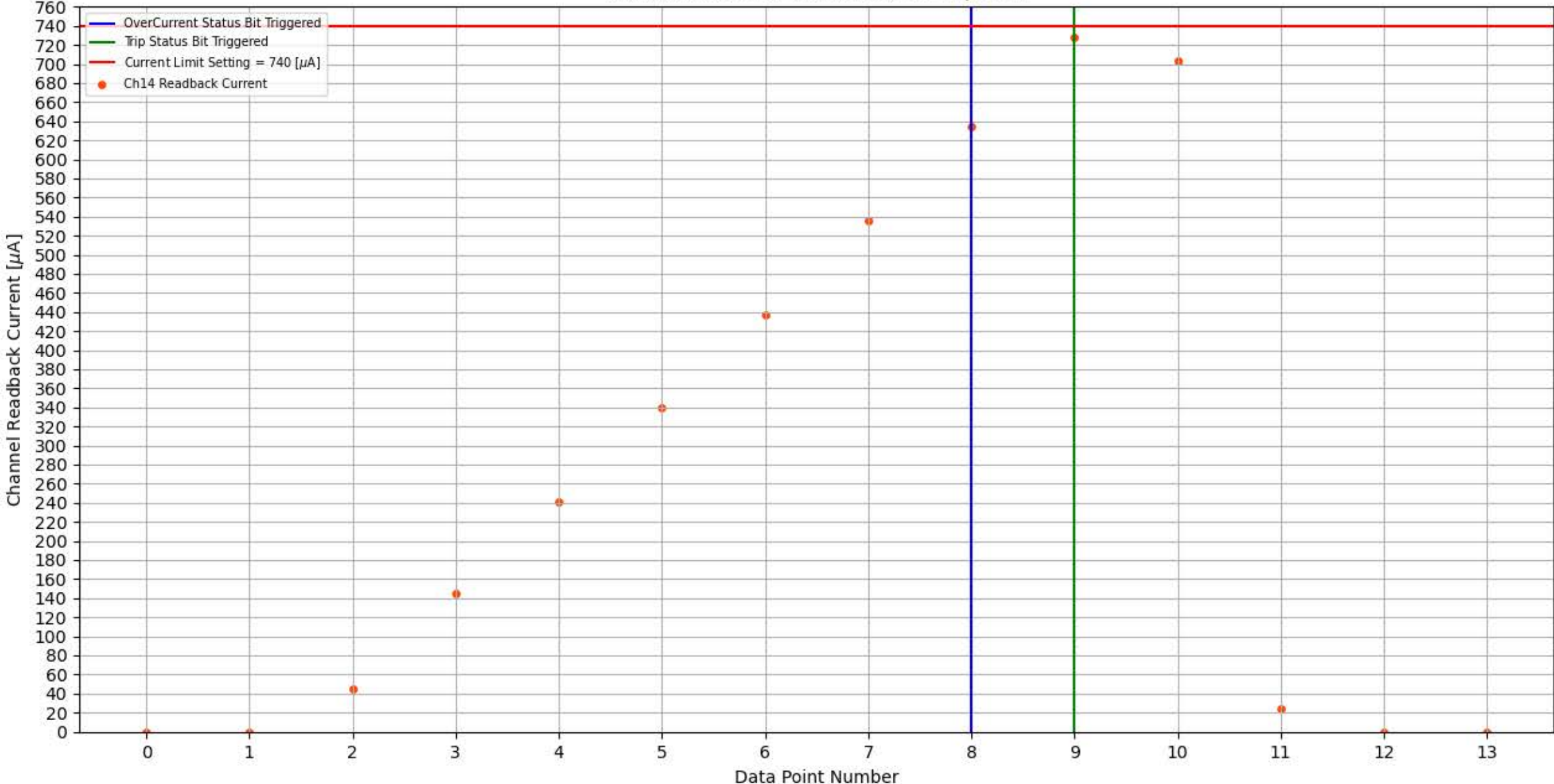
Module 356, Slot 1, Channel 14 Trip Test
