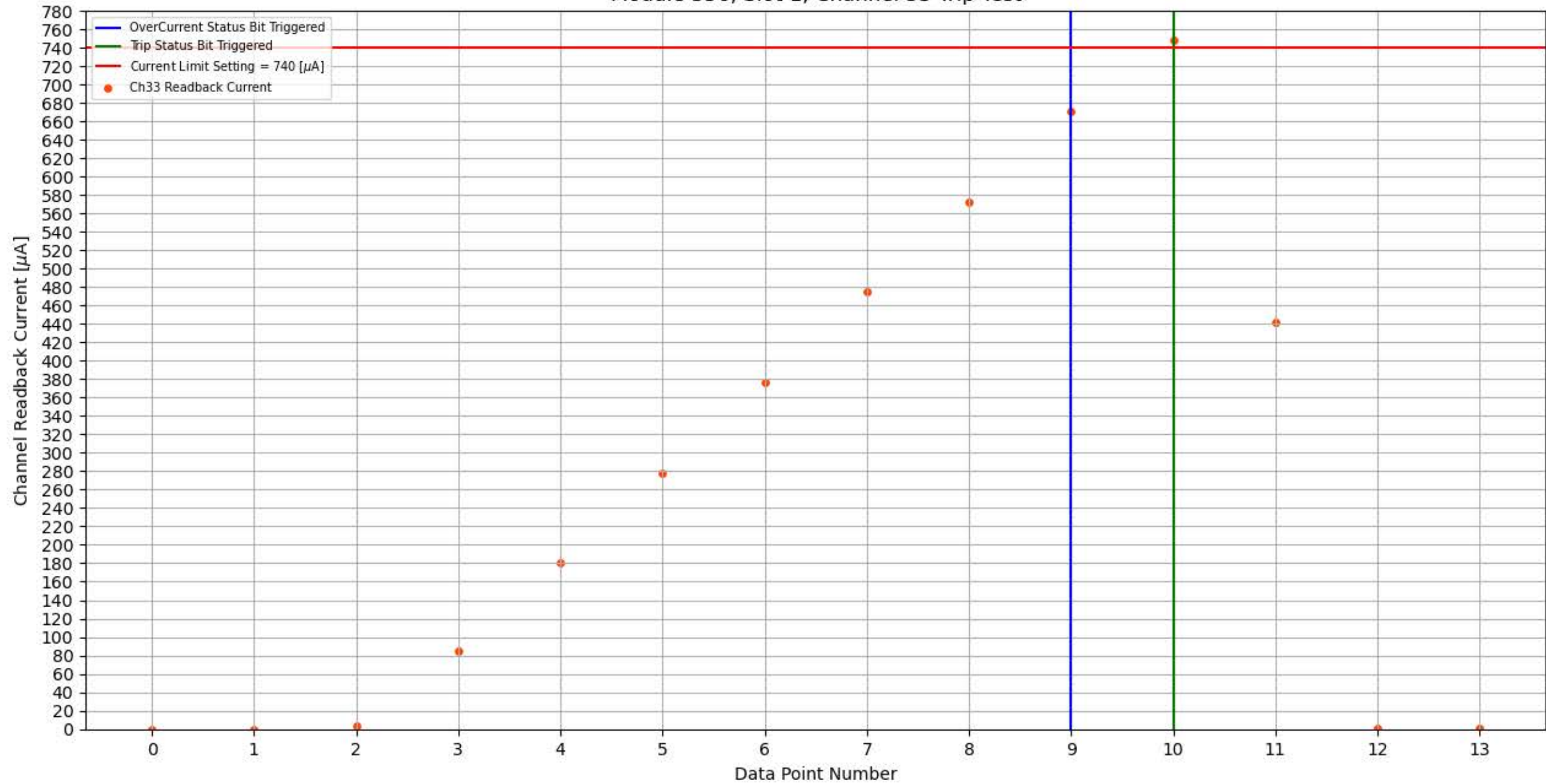
Module 356, Slot 1, Channel 33 Trip Test
