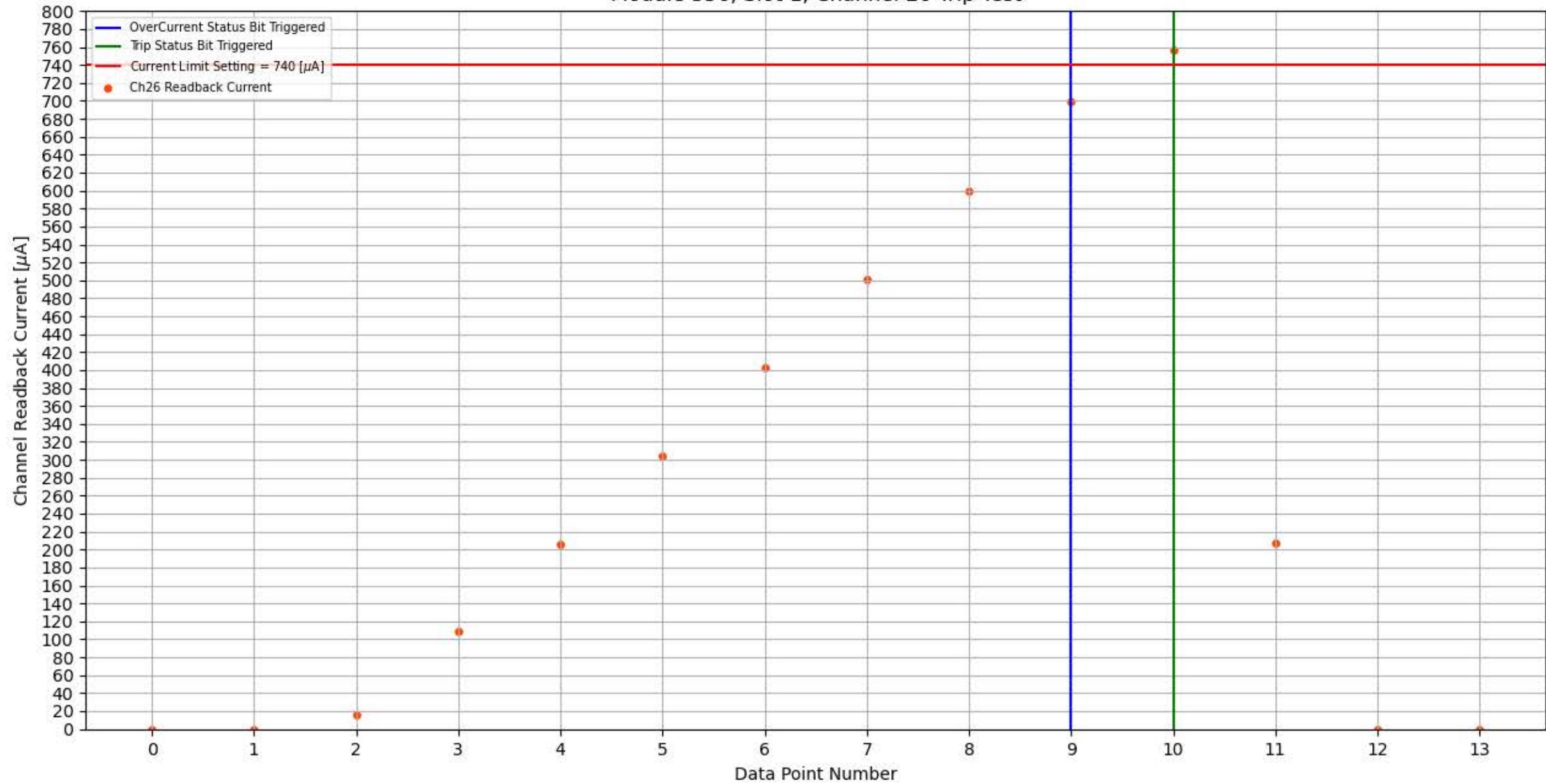
Module 356, Slot 1, Channel 26 Trip Test
