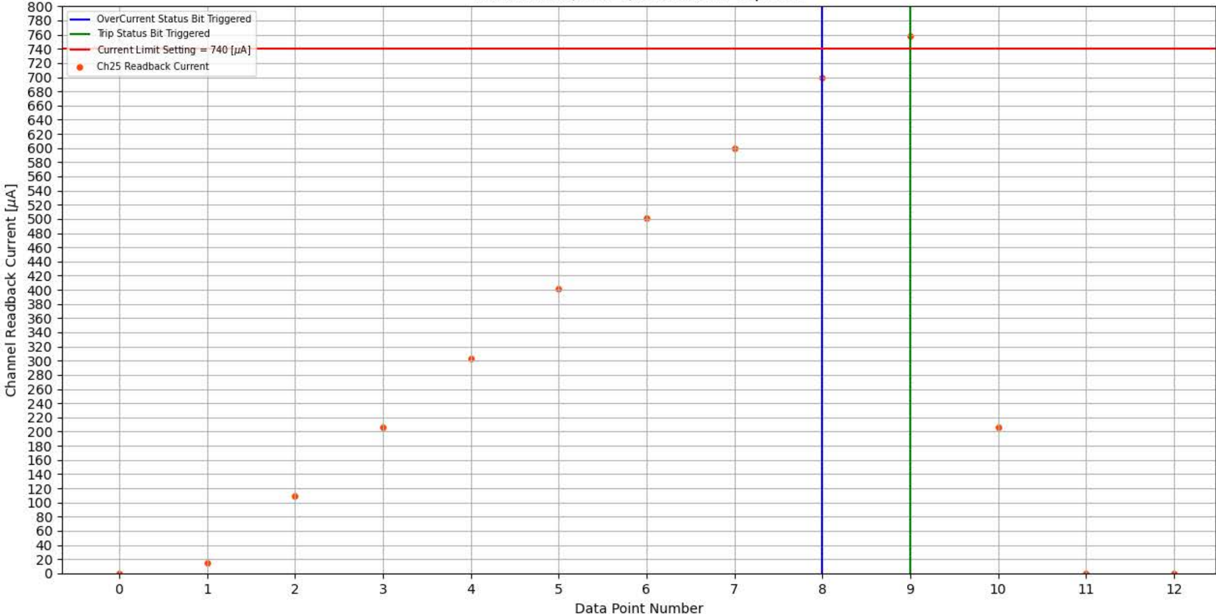
Module 356, Slot 1, Channel 25 Trip Test
