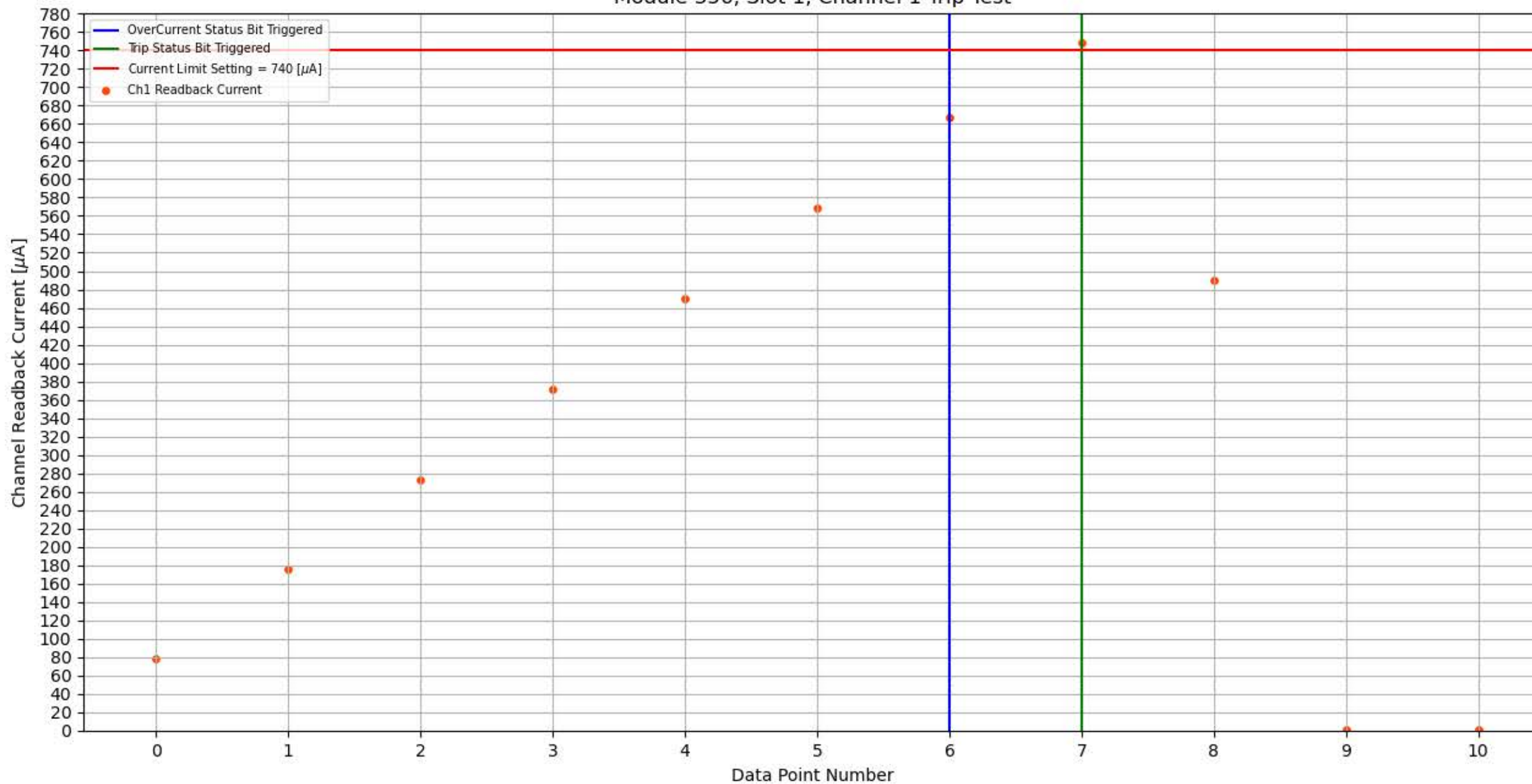
Module 356, Slot 1, Channel 1 Trip Test
