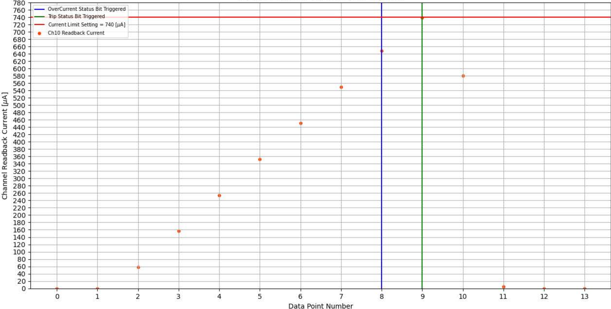
Module 356, Slot 1, Channel 10 Trip Test
