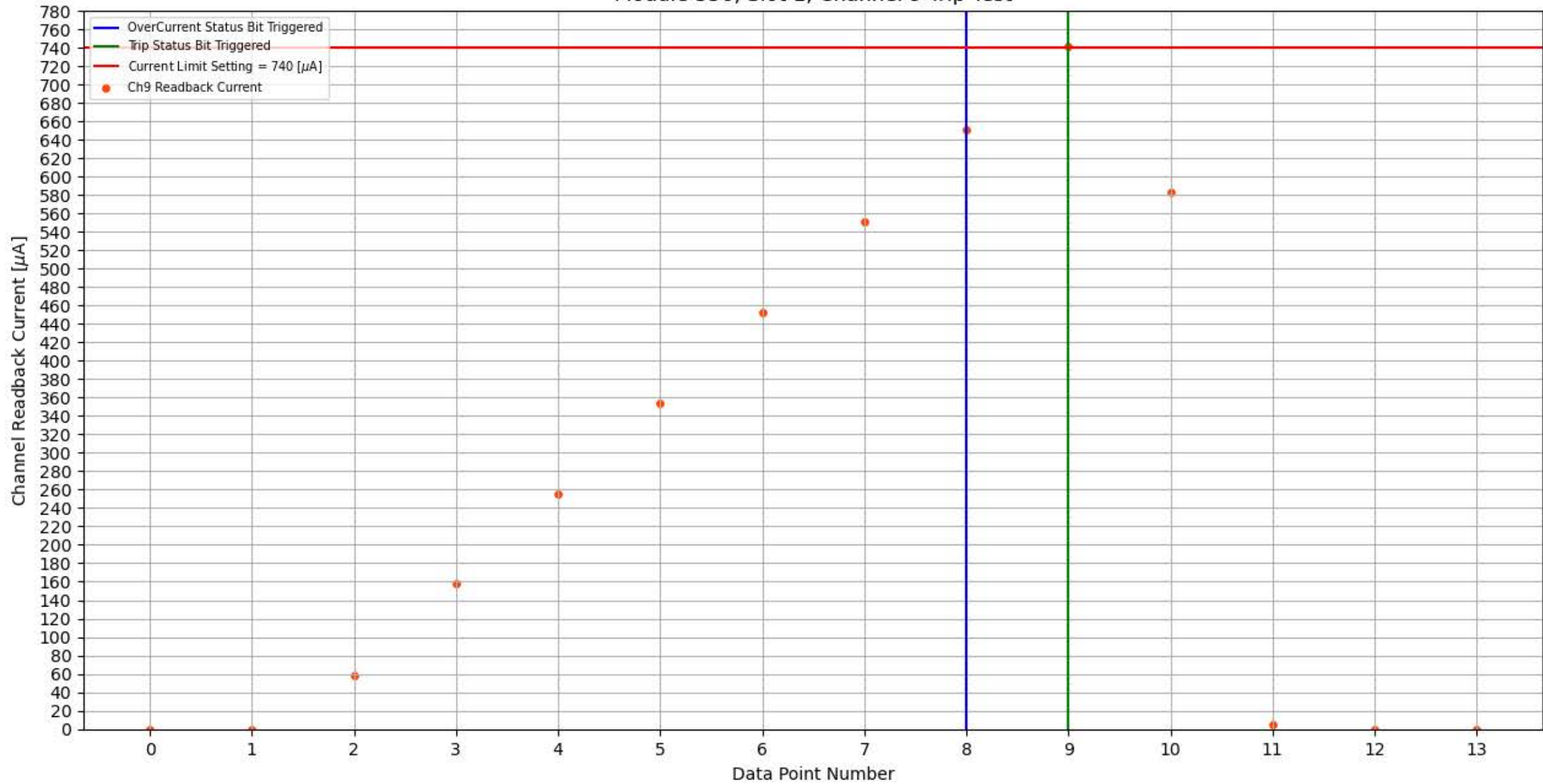
Module 356, Slot 1, Channel 9 Trip Test
