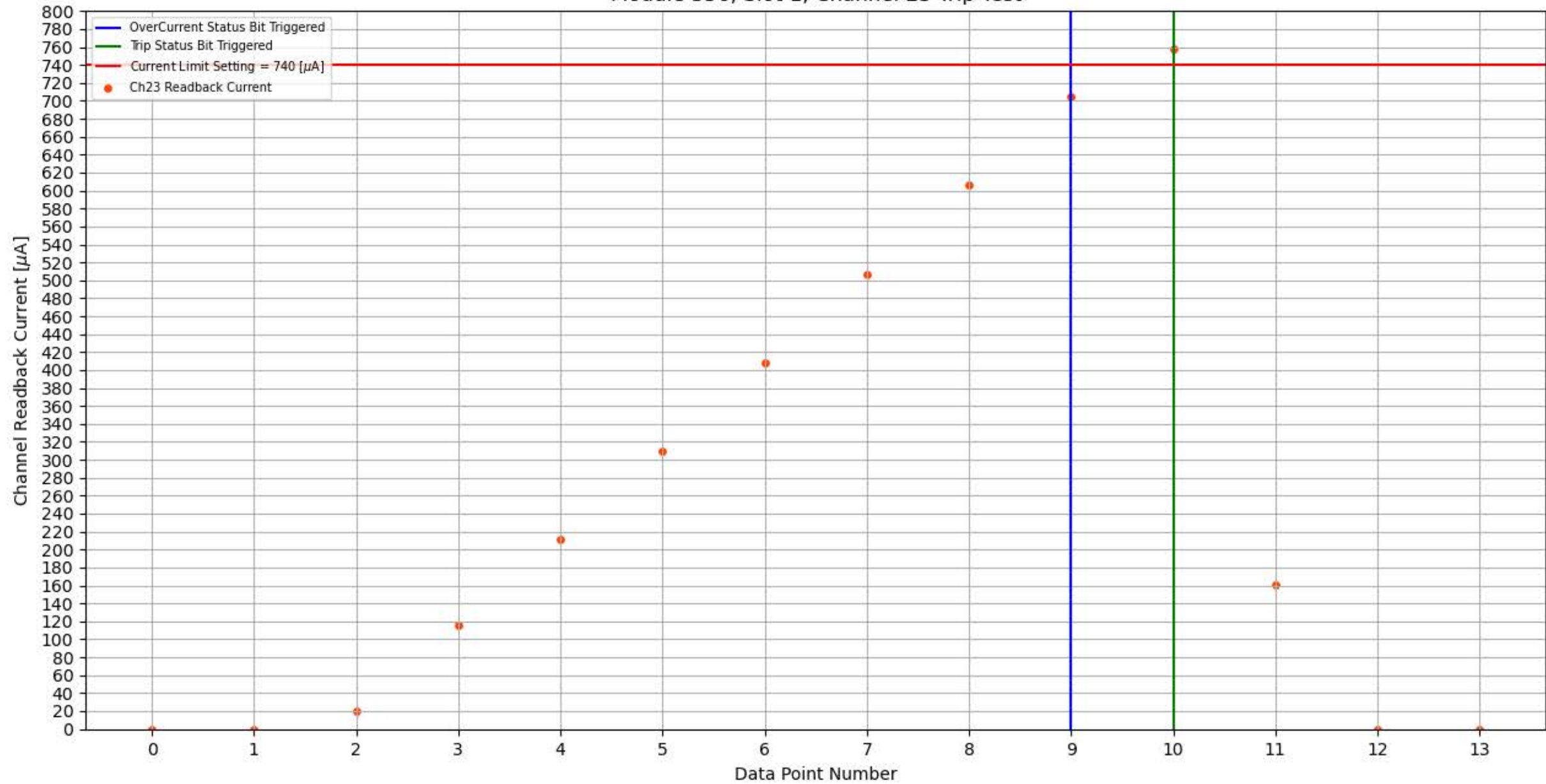
Module 356, Slot 1, Channel 23 Trip Test
