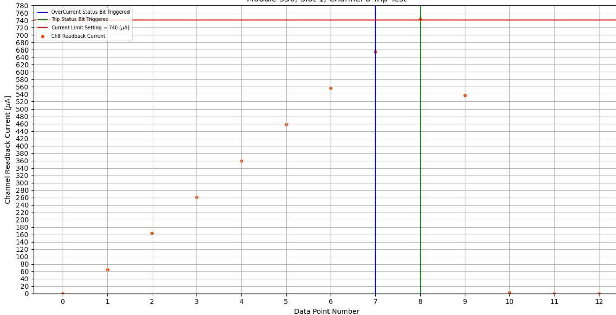
Module 356, Slot 1, Channel 8 Trip Test
