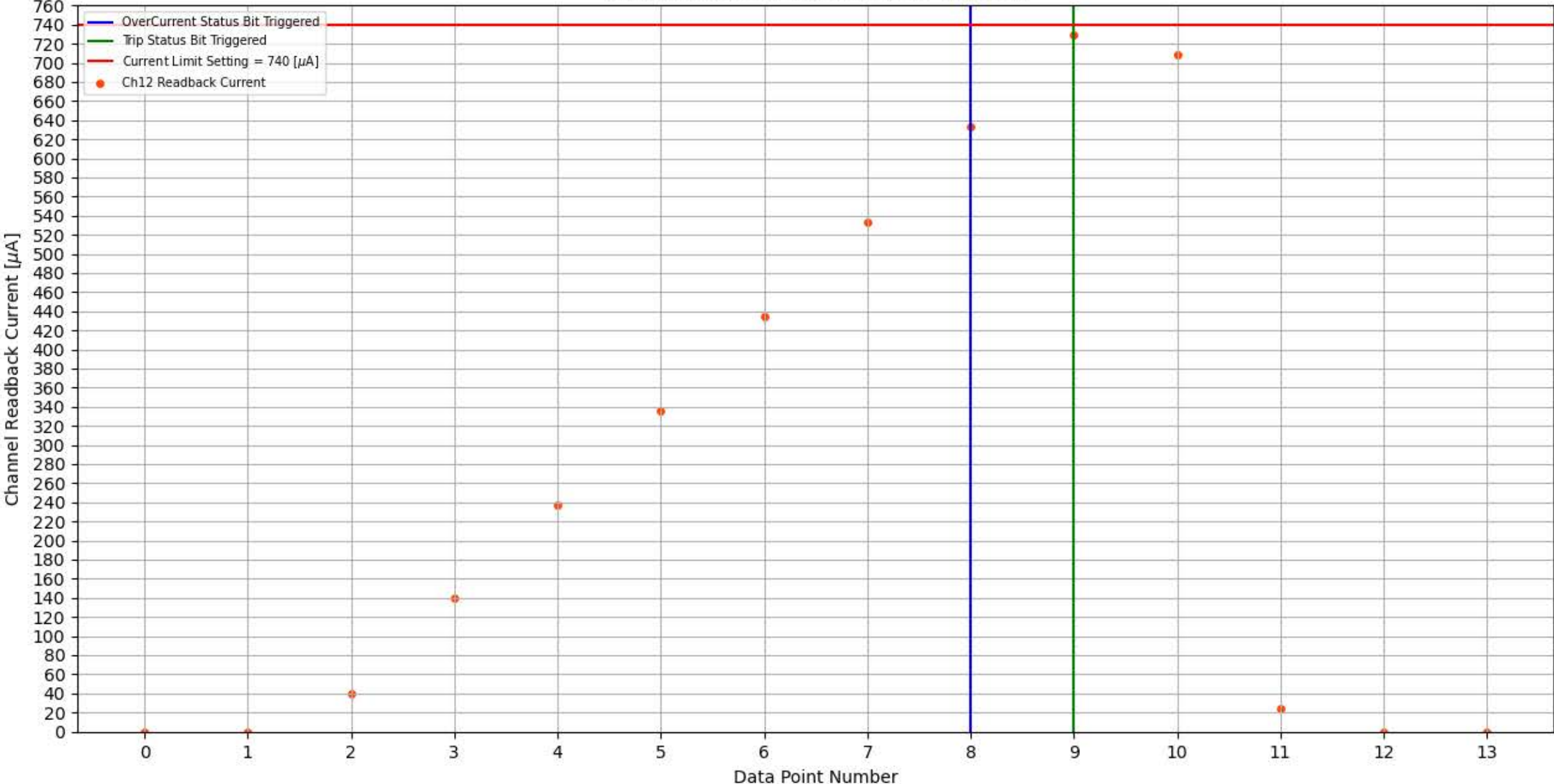
Module 356, Slot 1, Channel 12 Trip Test
