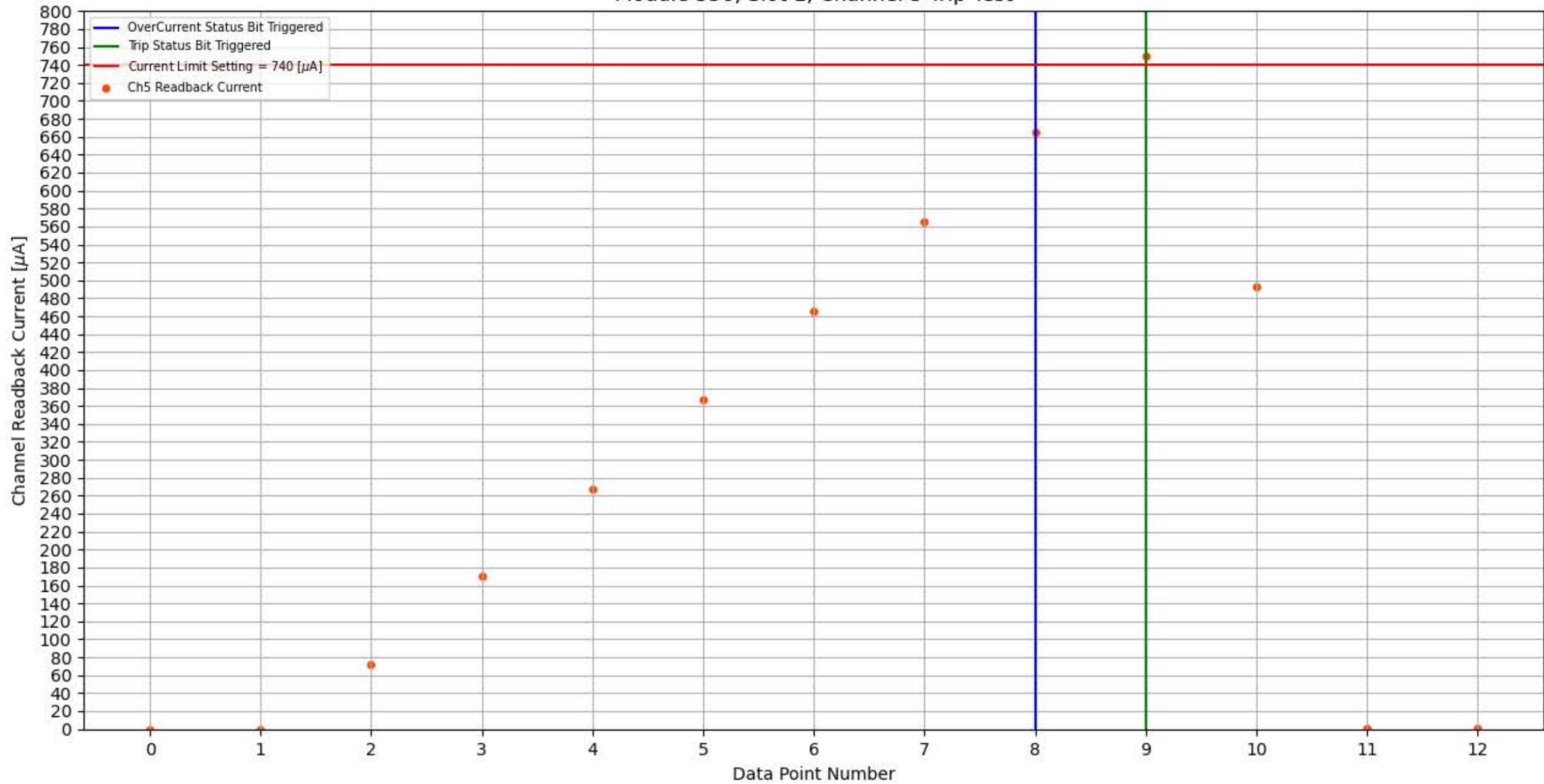
Module 356, Slot 1, Channel 5 Trip Test
