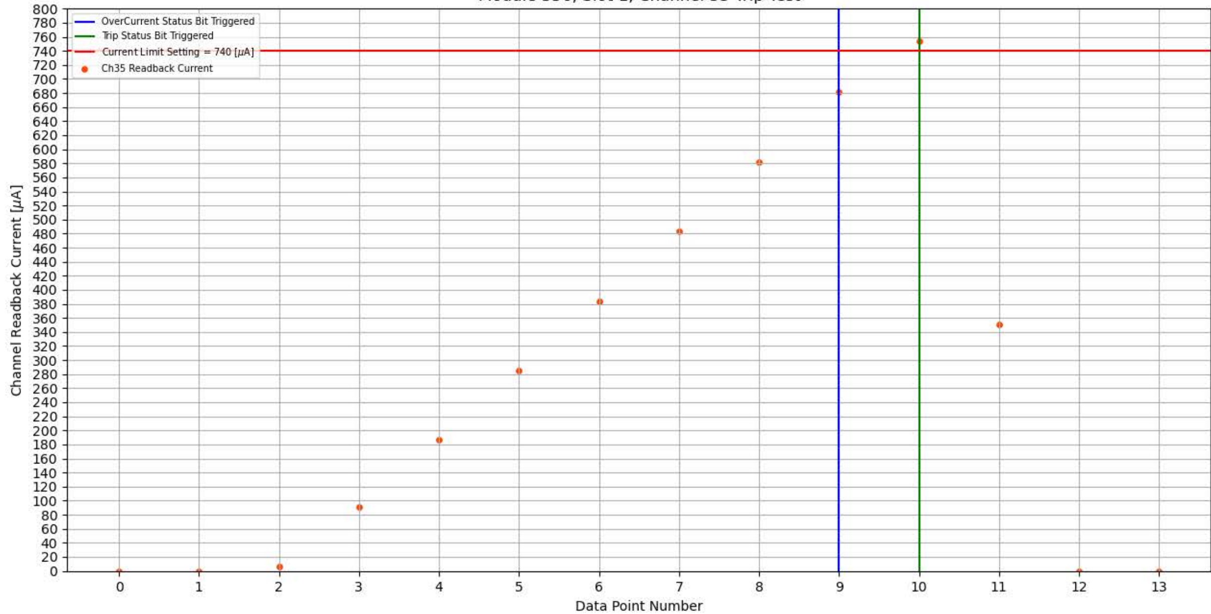
Module 356, Slot 1, Channel 35 Trip Test
