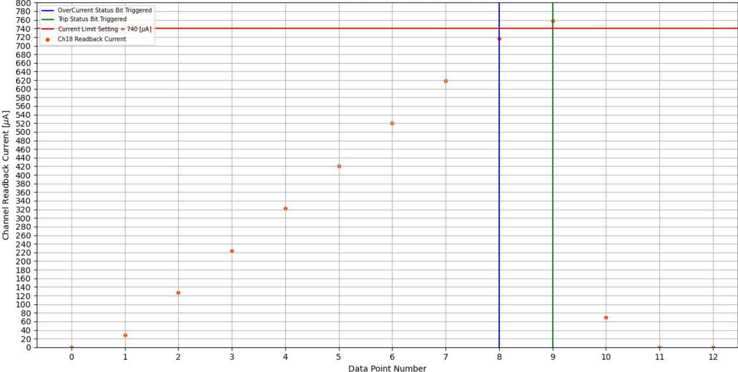
Module 356, Slot 1, Channel 18 Trip Test
