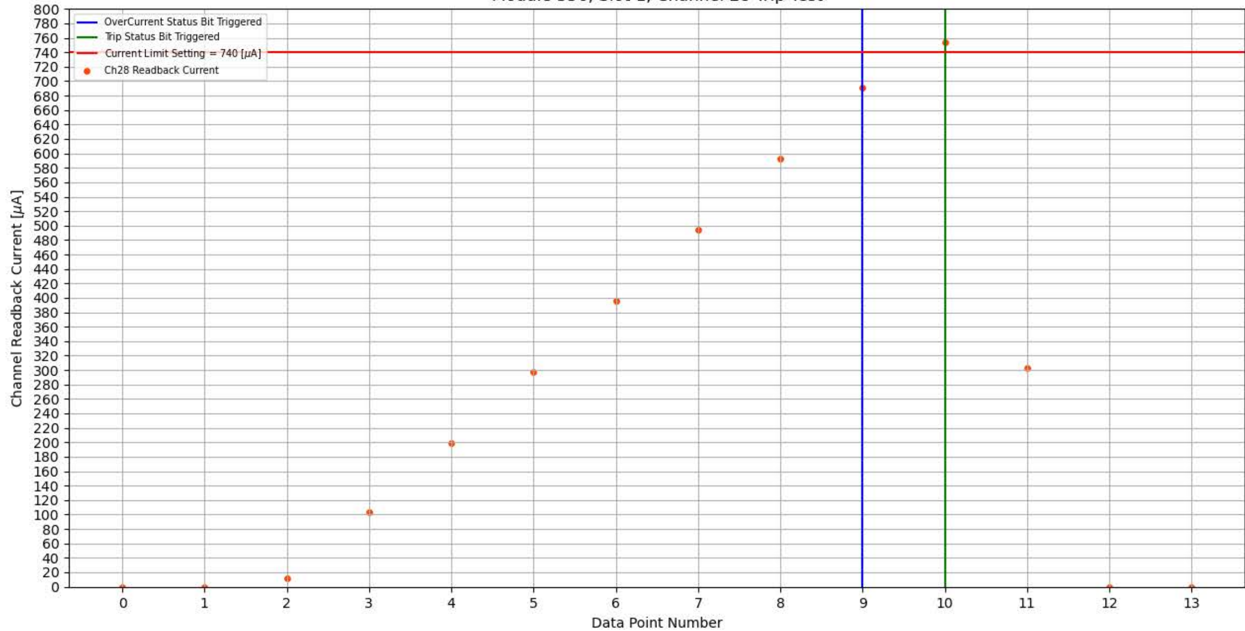
Module 356, Slot 1, Channel 28 Trip Test
