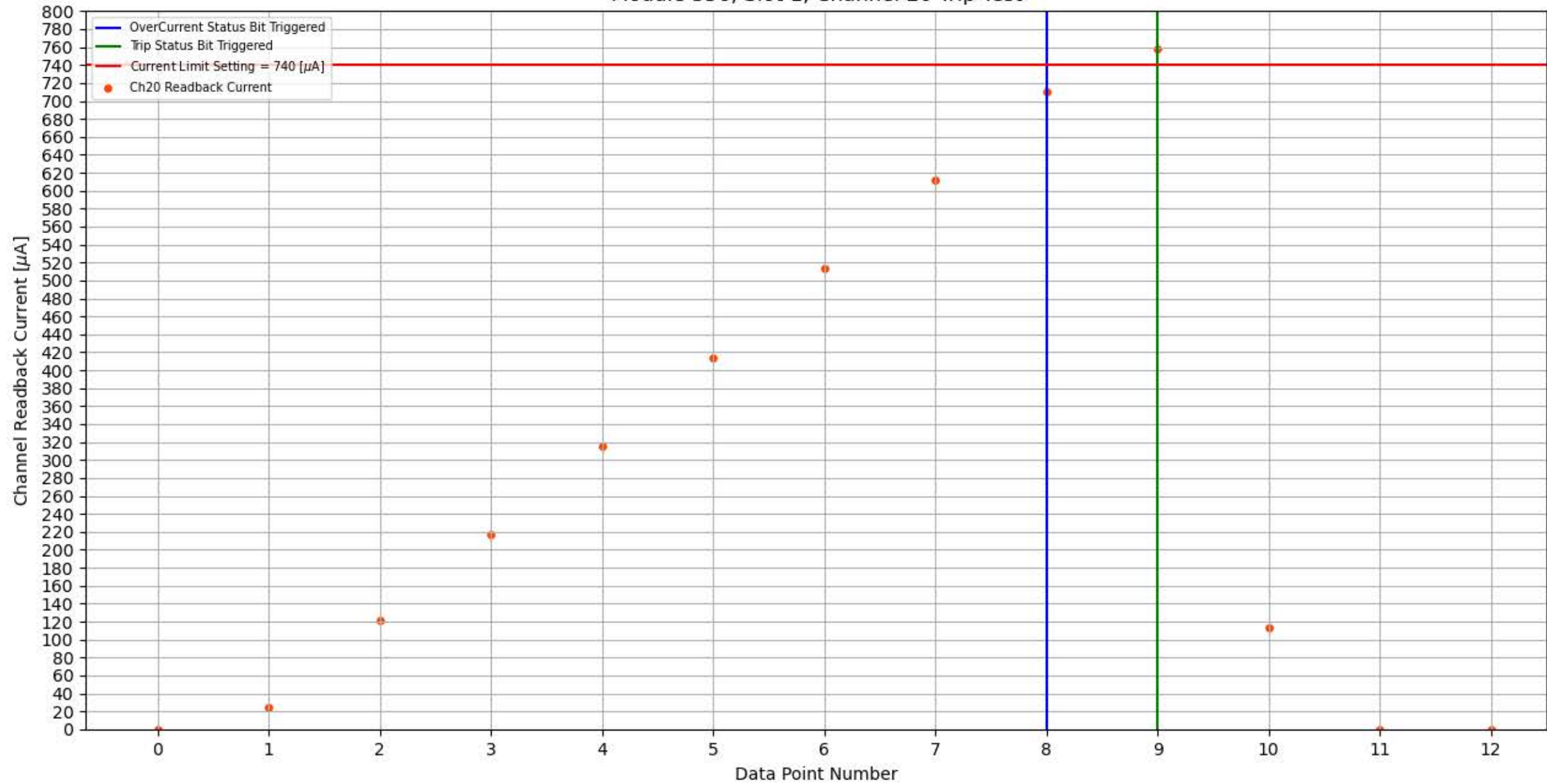
Module 356, Slot 1, Channel 20 Trip Test
