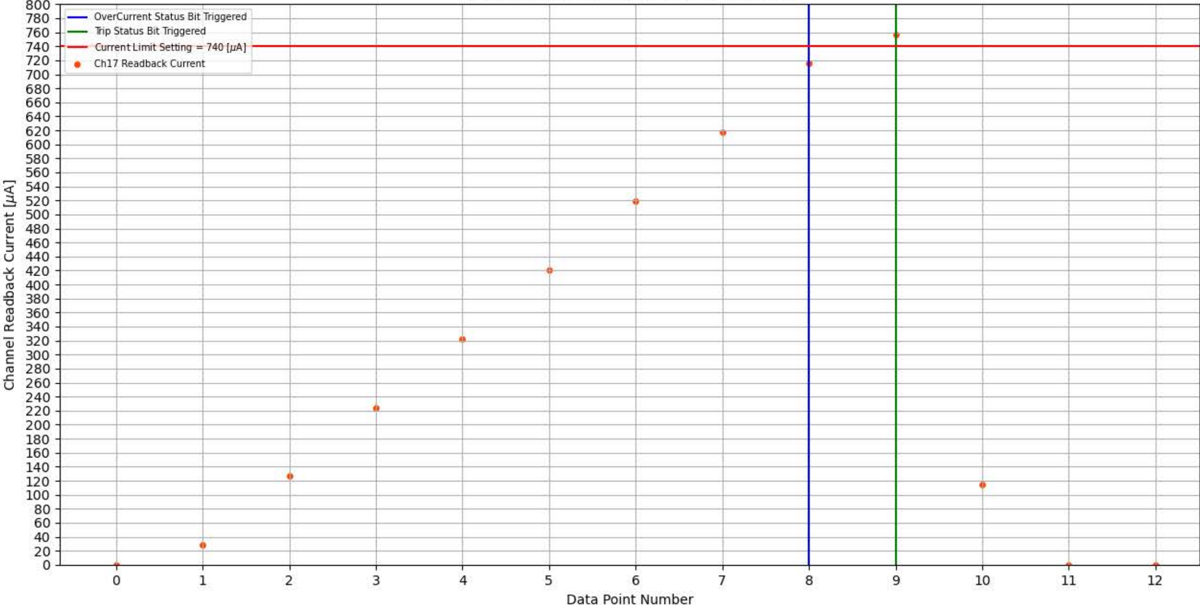
Module 356, Slot 1, Channel 17 Trip Test
