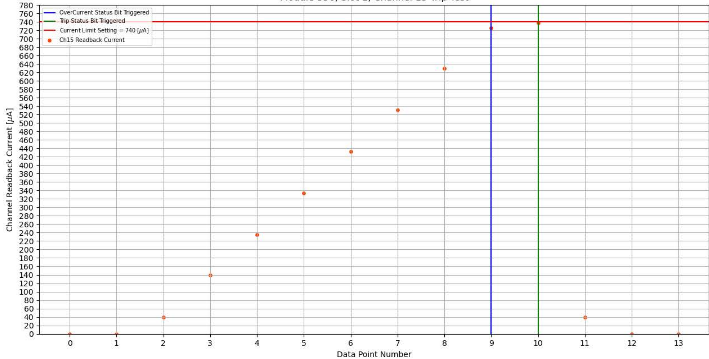
Module 356, Slot 1, Channel 15 Trip Test
