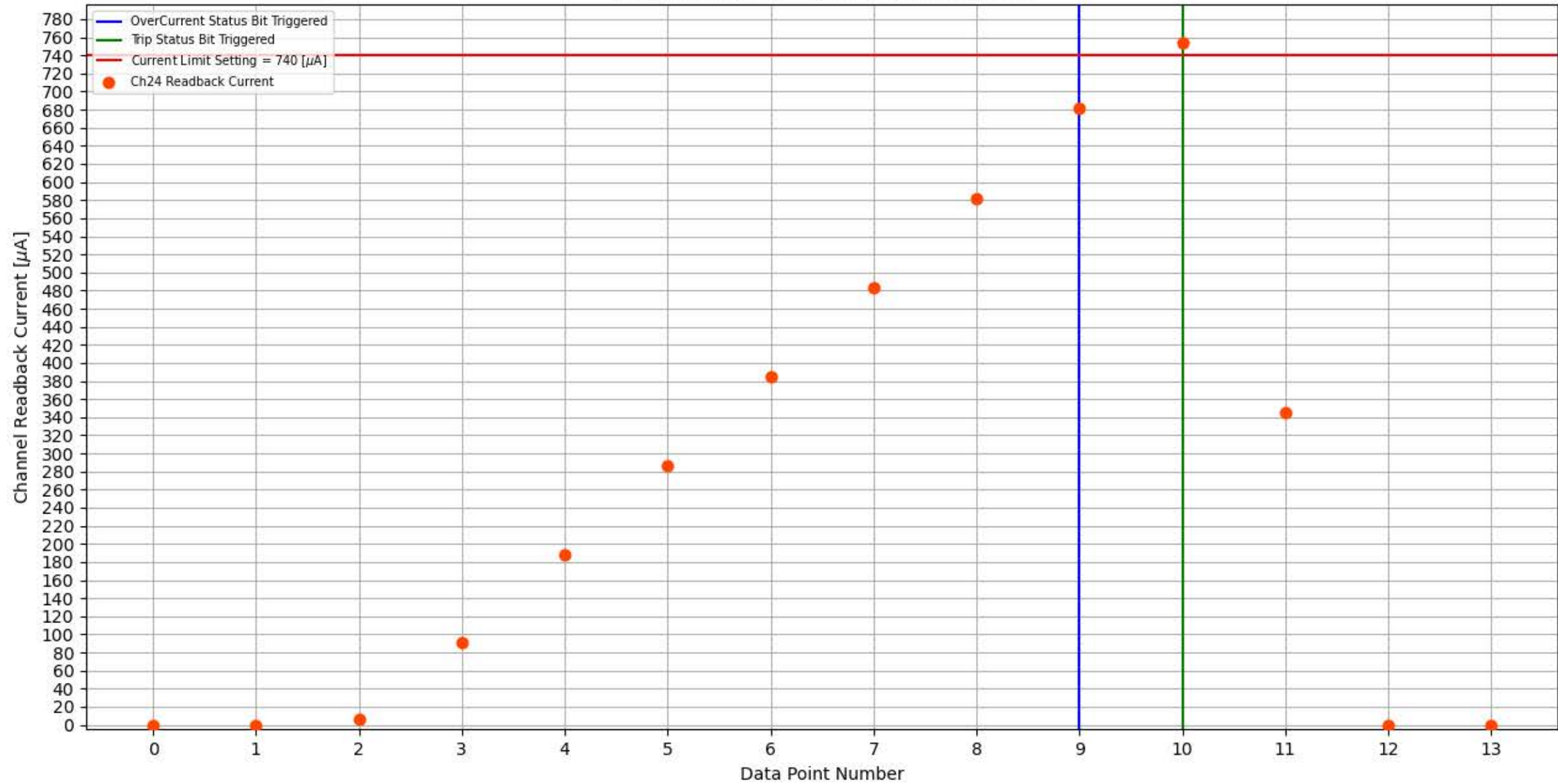
Module 356, Slot 1, Channel 24 Trip Test
