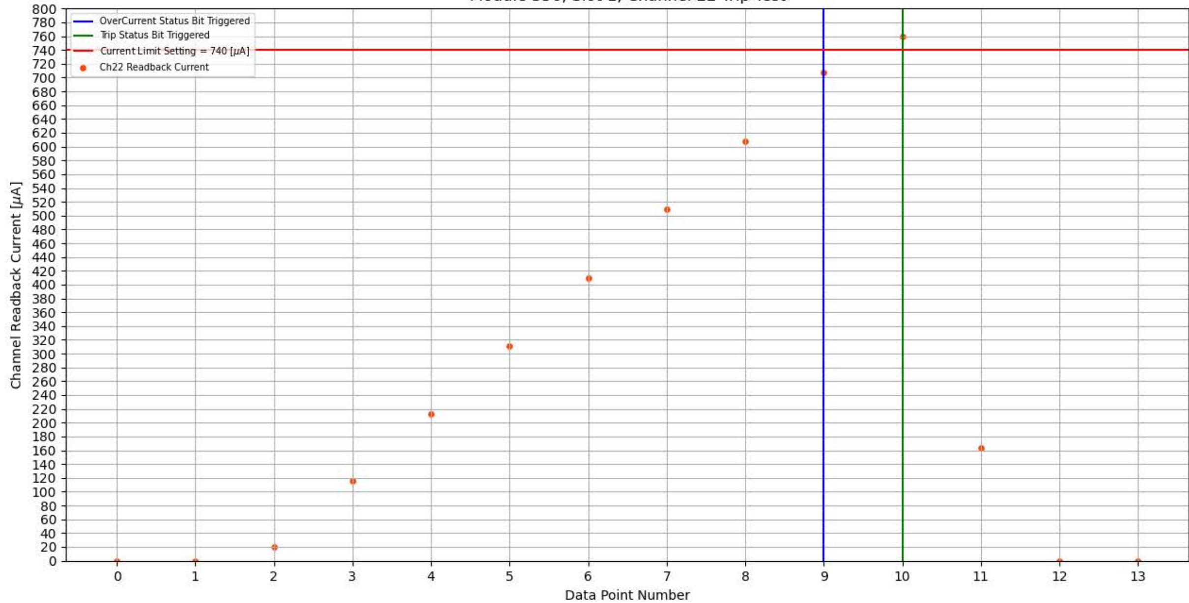
Module 356, Slot 1, Channel 22 Trip Test
